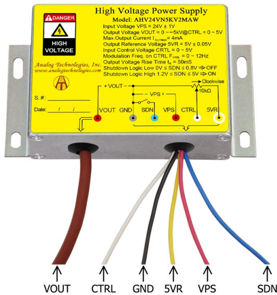
Figure 2. The Connecting Lead Wires of AHV24VN5KV2MAW
