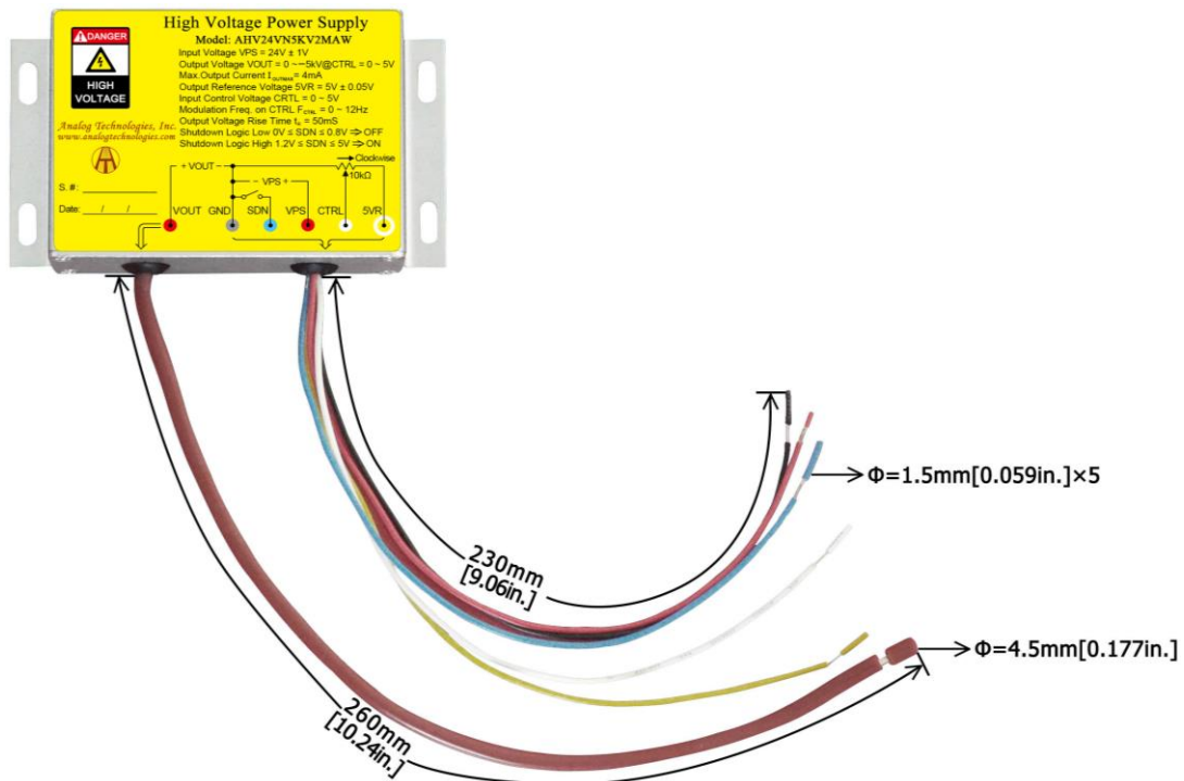
Figure 13. Connecting Lead Wires of AHV24VN5KV2MAW
