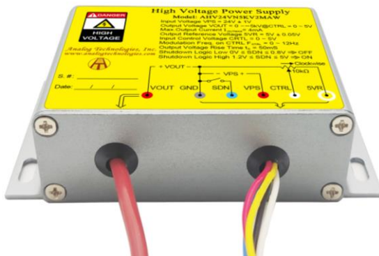
Figure 1.2. Side View
